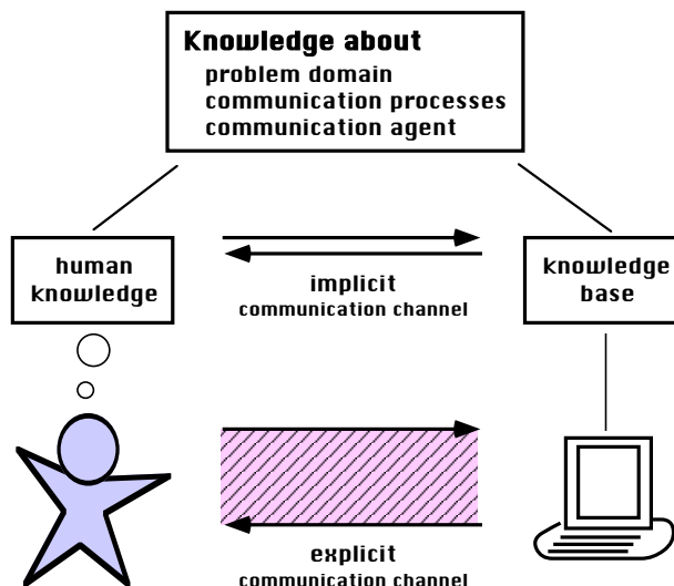
Figure 2: Knowledge-Based HCI
