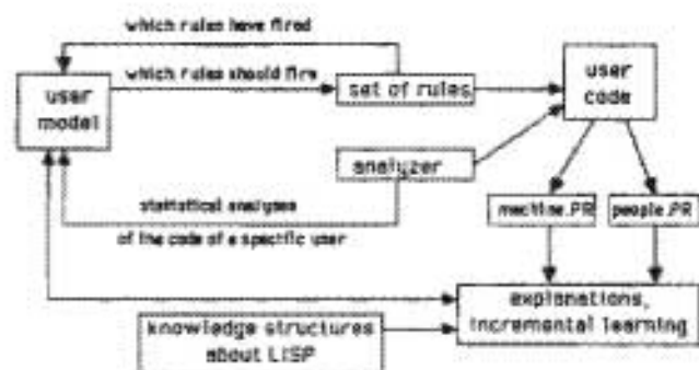
Figure 4-3: The Architecture of the USP-CRMC
