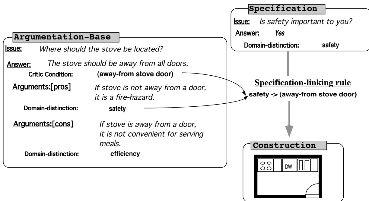
Figure 6. Derivation of the Specification-Linking Rules. The domain distinction associated with a specification item is paired with a matching pro or con argument in the hypermedia issue base. The critic condition associated with an answer is linked with the domain distinction to form a specific critic rule.
